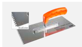
Schlüter®-TROWEL Strana 339
