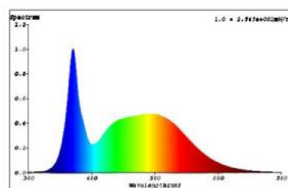
Spectral power distribution at 6500K
