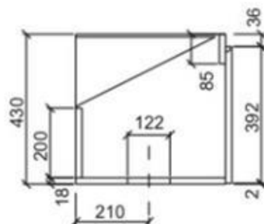
Bokorys
