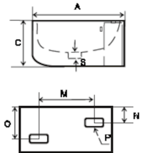
BIDE VIEW
